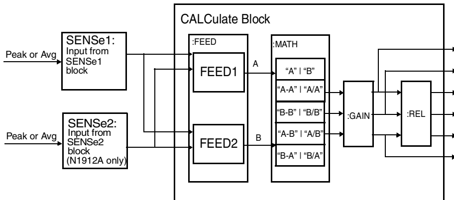
Figure 3-2 CALCulate Block
